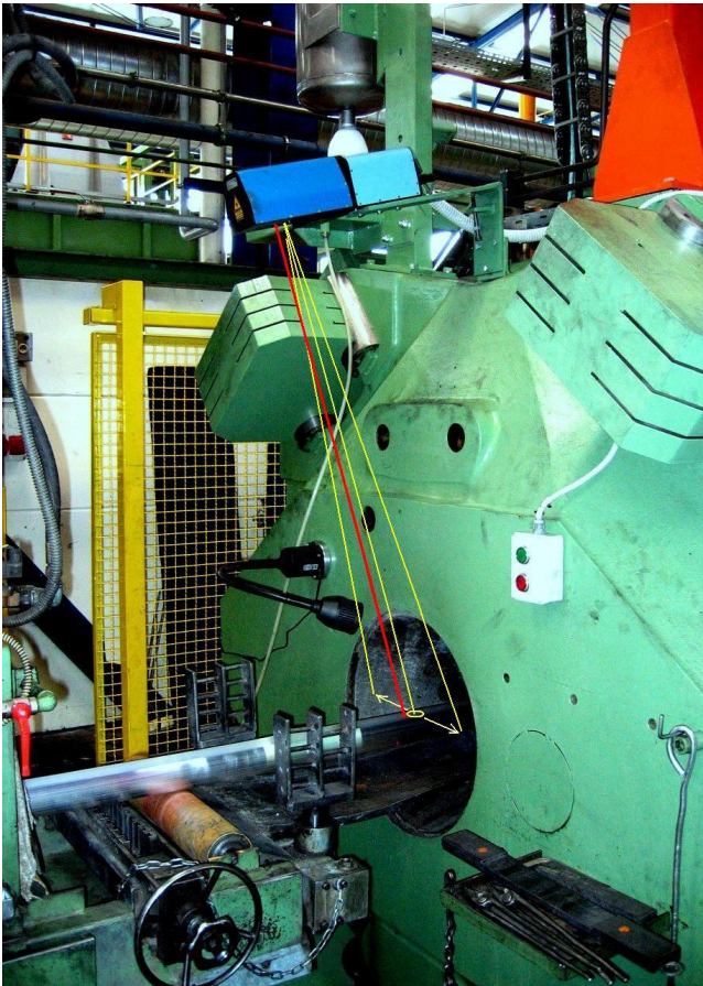
Aluminum Profile Sensor with scanner
