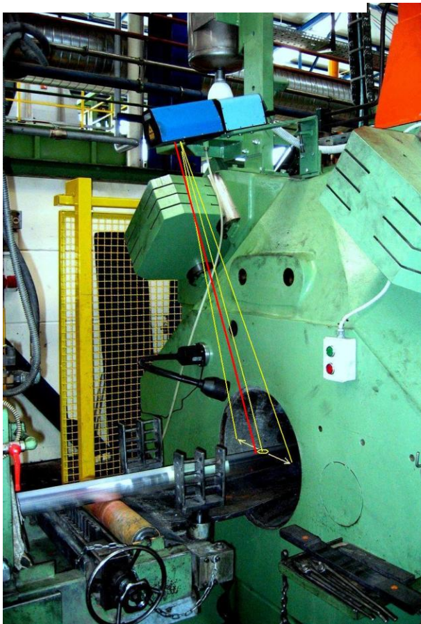
Aluminum Profile Sensor with scanner
